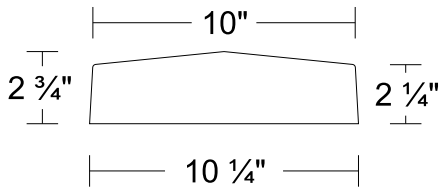
WC507-10.25x2.75x36
