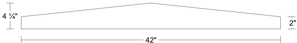
WC507-42x4.25
