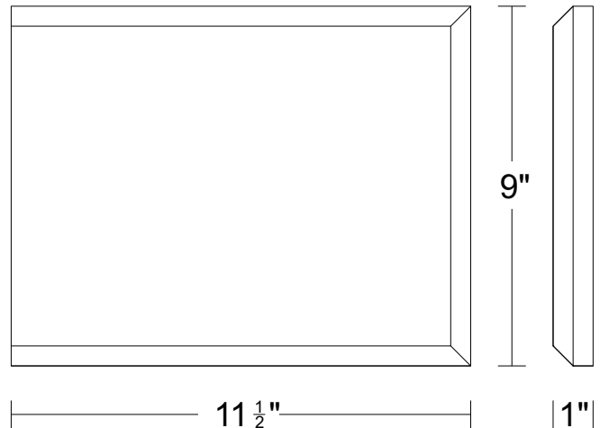
QN1-12x9-E Front View
